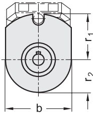
Execution for linear actuators ø18, 30, 40, 50
